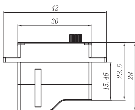
Xact SG5101H with Horizontal Tab
