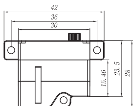
Xact SG5101H with Vertical Tab (for Flat builds)
