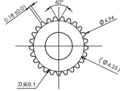
25T-5mm Output Shaft Spline
